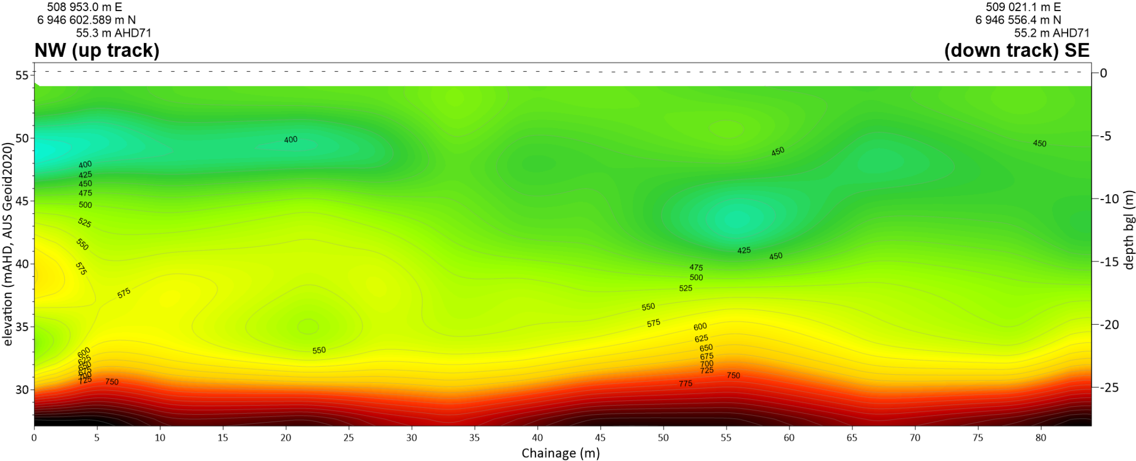
Seismic Line MASW AU-GP 102
